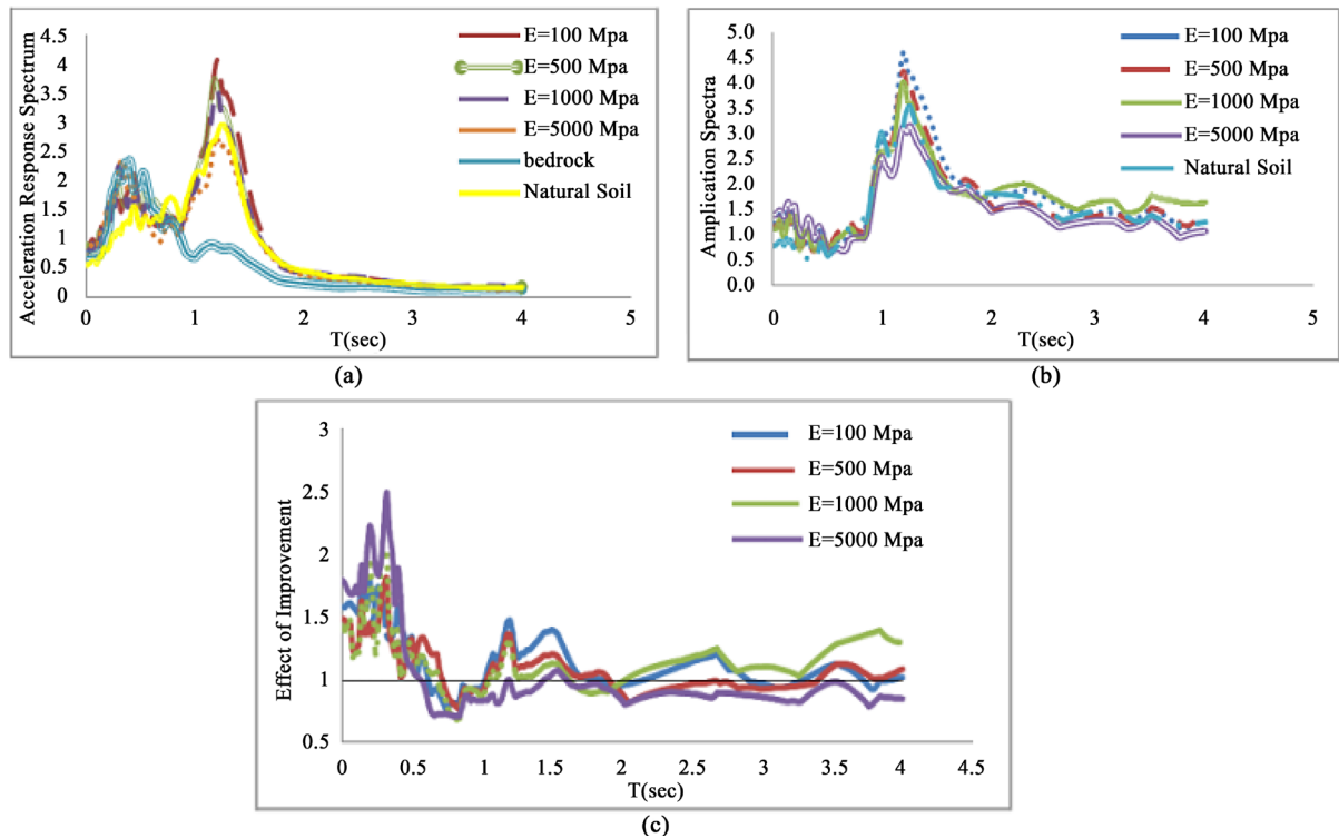
Figure 8. Comparison of seismic response on the surface of the natural ground and its improvement under far-fault Loma Prieta earthquake with PGA = 0.7 g (a) elastic response spectra, (b) amplification of S_a , (c) the effect of improvement on S_a .
