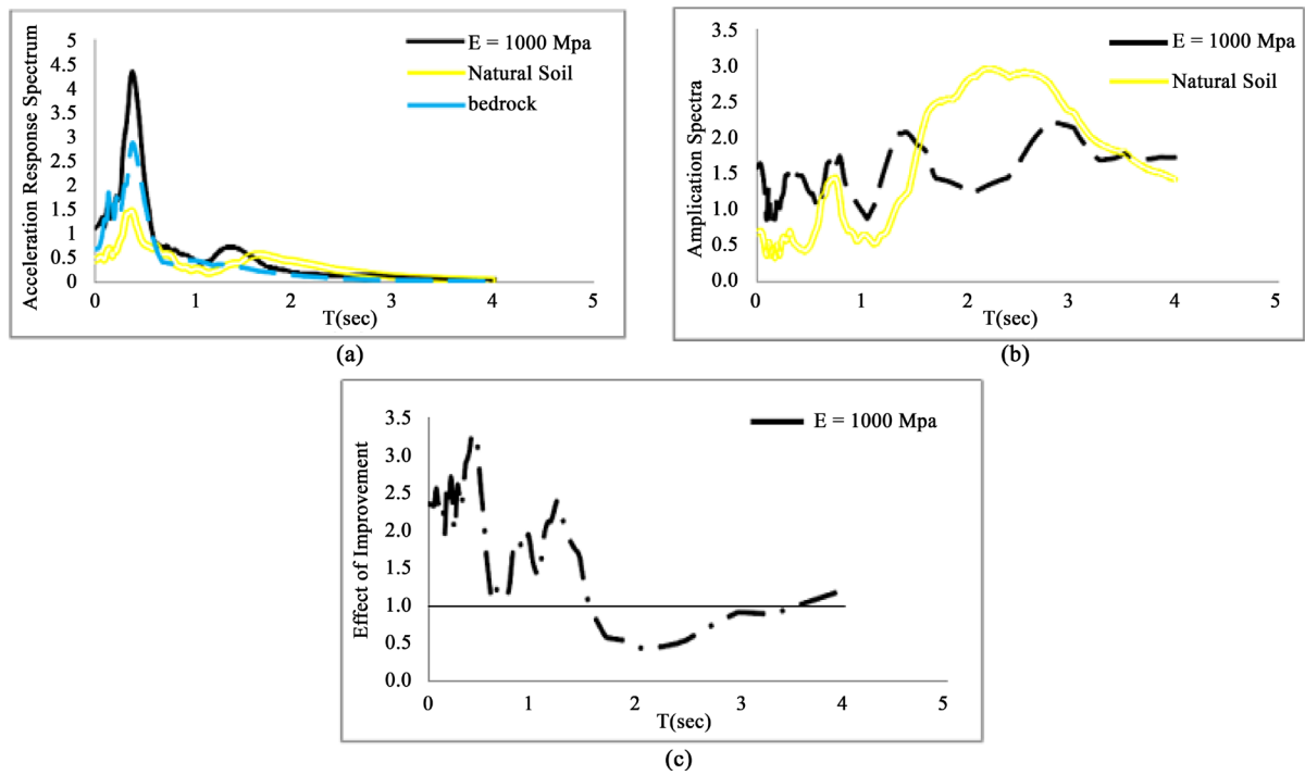
Figure 15. Comparison of seismic response on the surface of the natural ground and its improvement under near-fault Loma Prieta earthquake with PGA = 0.7 g: (a) elastic response spectra, (b) amplification of S_a , (c) the effect of improvement on S_a .
