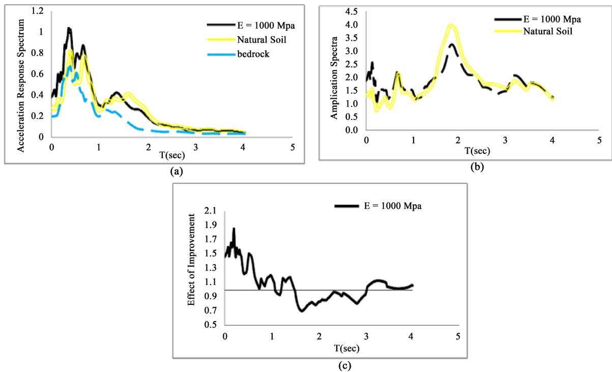
Figure 16. Comparison of seismic response on the surface of the natural ground and its improvement under far-fault Loma Prieta earthquake with PGA = 0.2 g: (a) elastic response spectra, (b) amplification of S_a , (c) the effect of improvement on S_a .
