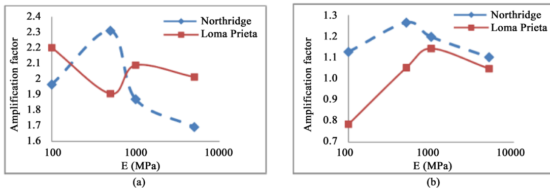
Figure 1. Amplification factor on the surface of improved grounds under near-fault earthquake with (a) PGA = 0.2 g and (b) PGA = 0.7 g.
