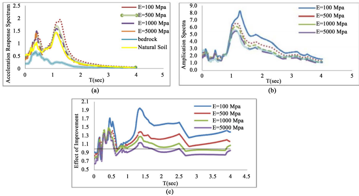
Figure 7. Comparison of seismic response on the surface of the natural ground and its improvement under far-fault Loma Prieta earthquake with PGA = 0.2 g (a) elastic response spectra, (b) amplification of S_a , (c) the effect of improvement on S_a .
