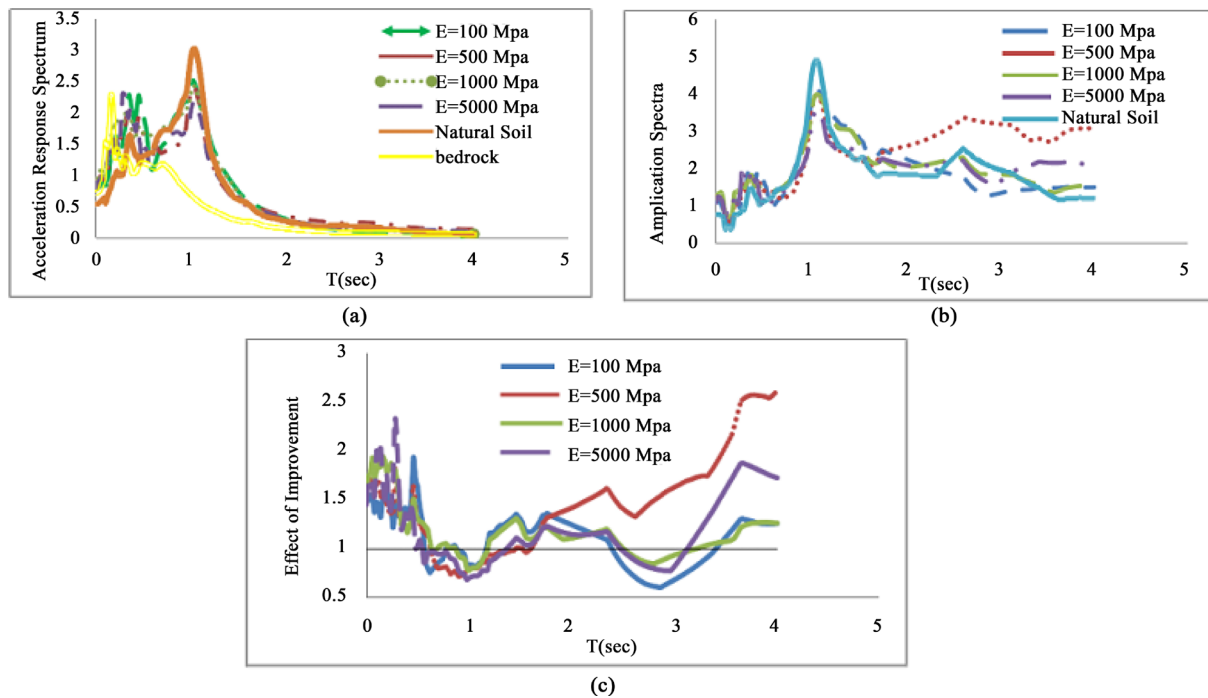
Figure 6. Comparison of seismic response on the surface of the natural ground and its improvement under near-fault Northridge earthquake with PGA = 0.7 g (a) elastic response spectra, (b) amplification of S_a , (c) the effect of improvement on S_a .
