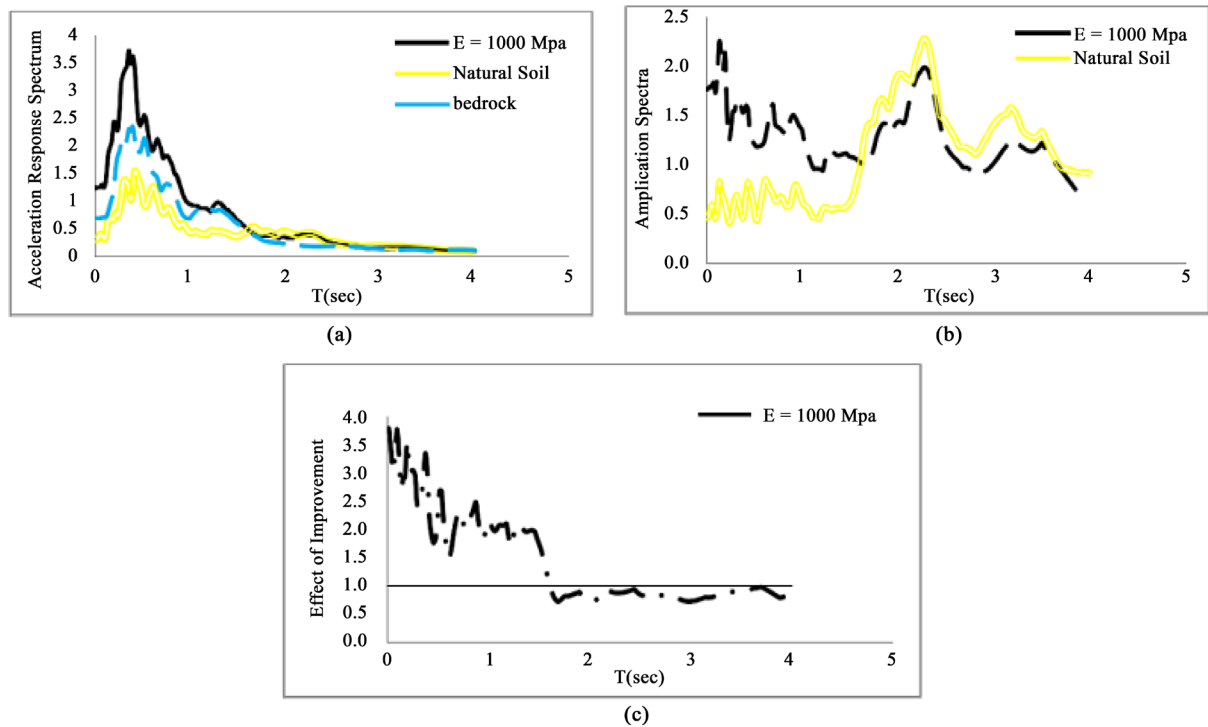
Figure 17. Comparison of seismic response on the surface of the natural ground and its improvement under far-fault Loma Prieta earthquake with PGA = 0.7 g: (a) elastic response spectra, (b) amplification of Sa, (c) the effect of improvement on Sa.
