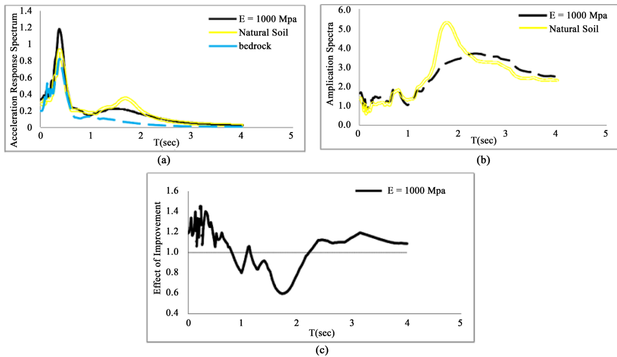
Figure 14. Comparison of seismic response on the surface of the natural ground and its improvement under near-fault Loma Prieta earthquake with PGA = 0.2 g: (a) elastic response spectra, (b) amplification of Sa, (c) the effect of improvement on Sa.
