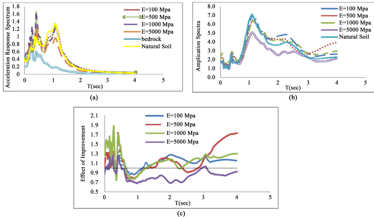
Figure 9. Comparison of seismic response on the surface of the natural ground and its improvement under far-fault Northridge earthquake with PGA = 0.2 g: (a) elastic response spectra, (b) amplification of S_a , (c) the effect of improvement on S_a .
