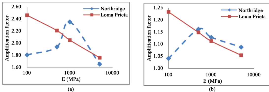
Figure 2. Amplification factor on the surface of the improved grounds under far-fault earthquake with: (a) PGA: 0.2 g and (b) PGA: 0.7 g.
