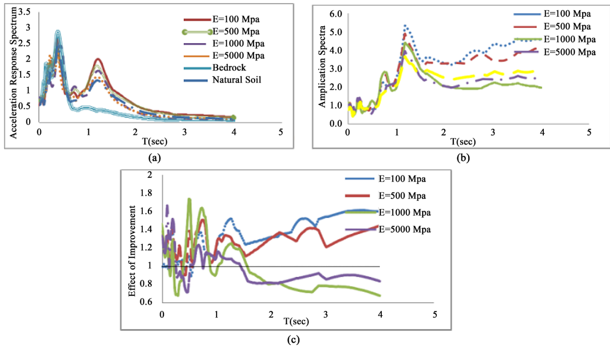
Figure 4. Comparison of seismic response on the surface of the natural ground and its improvement under near-fault Loma Prieta earthquake with PGA = 0.7 g: (a) elastic response spectra, (b) amplification of Sa, (c) the effect of improvement on Sa.
