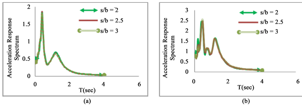
Figure 11. Acceleration response spectra for different pile distance ratios under near-fault Loma Prieta Earthquake with: (a) PGA = 0.2 g and (b) PGA = 0.7 g.
