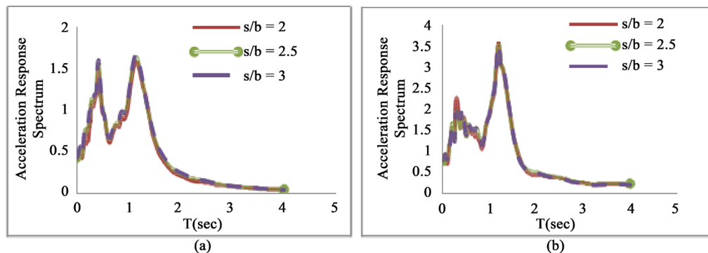
Figure 12. Acceleration response spectra for different pile distance ratios under far-fault Loma Prieta Earthquake with: (a) PGA = 0.2 g & (b) PGA = 0.7 g.
