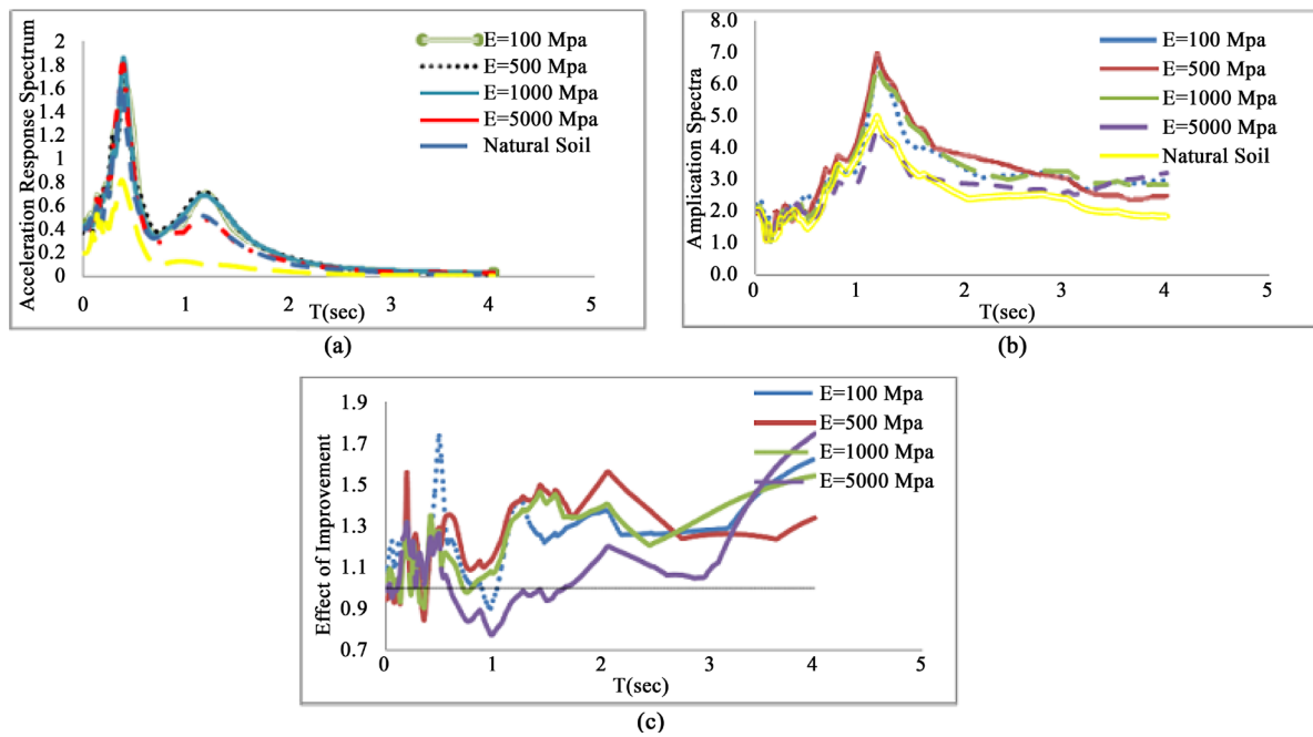
Figure 3. Comparison of seismic response on the surface of the natural ground and its improvement under near-fault Loma Prieta earthquake with PGA = 0.2 g: (a) elastic response spectra, (b) amplification of Sa, (c) the effect of improvement on Sa.
