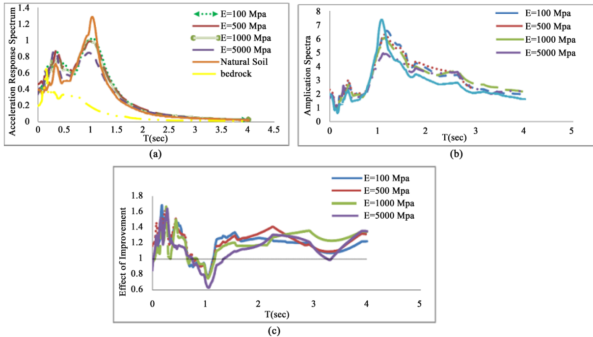
Figure 5. Comparison of seismic response on the surface of the natural ground and its improvement under near-fault Northridge earthquake with PGA = 0.2 g (a) elastic response spectra, (b) amplification of S_a , (c) the effect of improvement on S_a .
