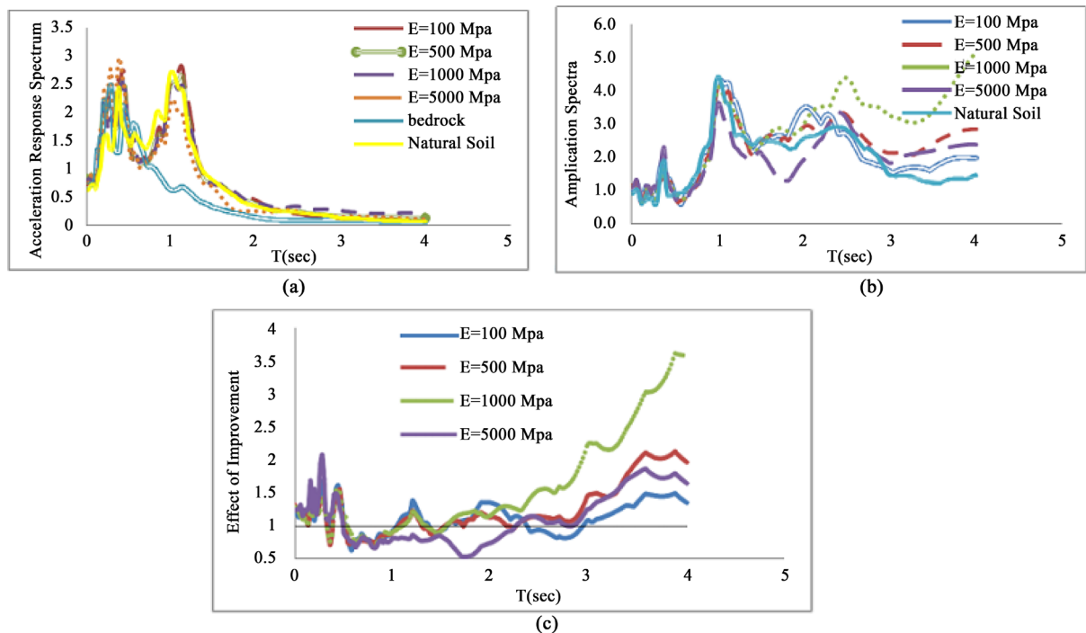
Figure 10. Comparison of seismic response on the surface of the natural ground and its improvement under far-fault Northridge earthquake with PGA = 0.7 g: (a) elastic response spectra, (b) amplification of S_a , (c) the effect of improvement on S_a .
