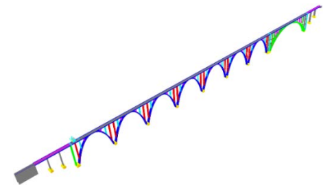
Papagaios Viaduct, Rumo Railways, SP, Brazil
