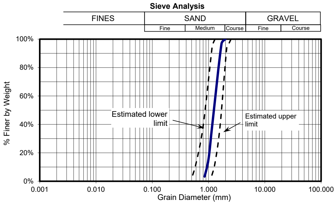
Figure 7: Estimated grain size distribution of backfill sand
