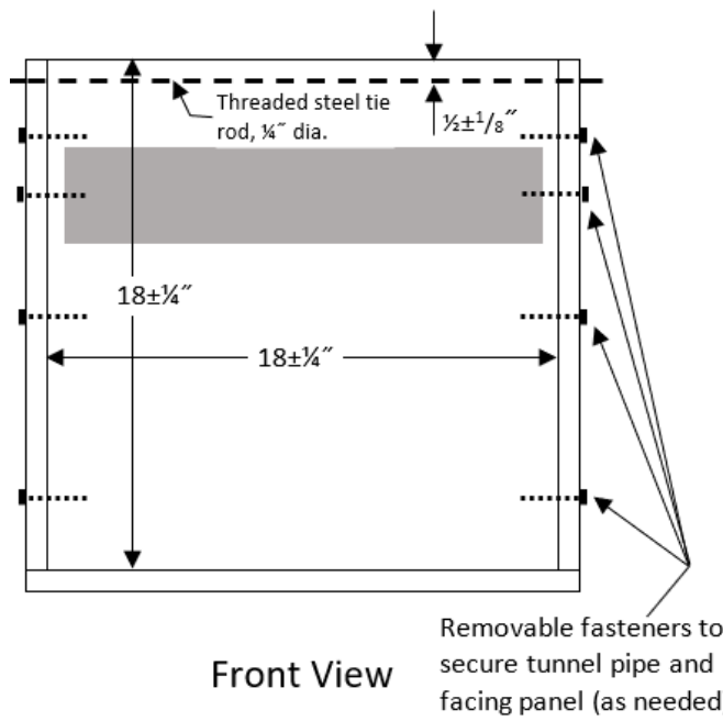
Figure 2: Sandbox dimensions (not to scale)
