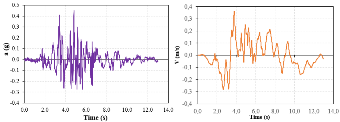
Figure 1: Acceleration (left) and integrated speed (right) of Loma Prieta earthquake.
