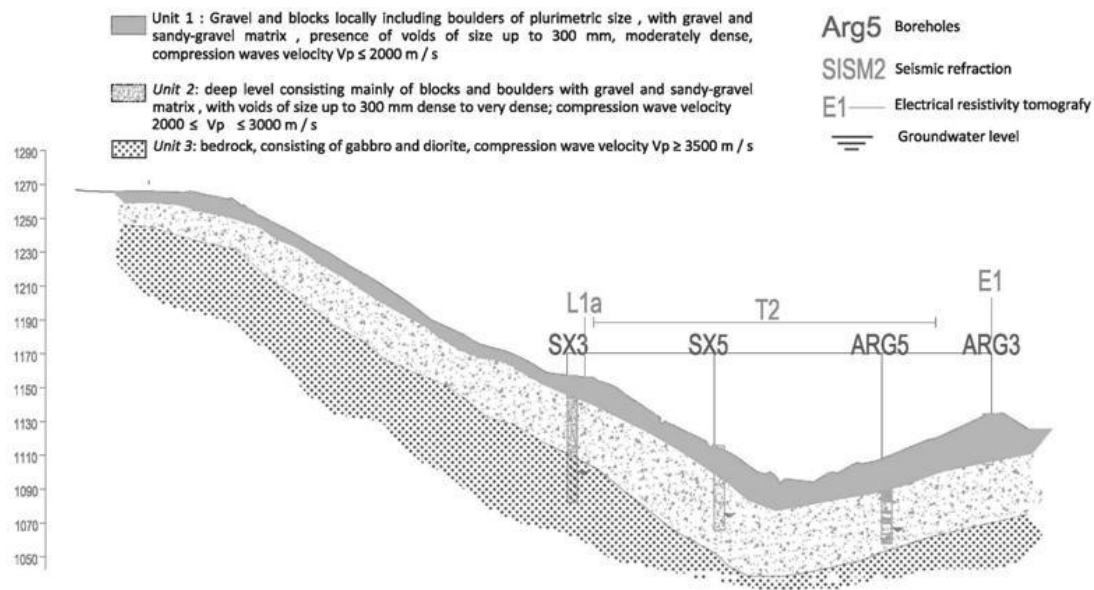
Figure 2 Typical geotechnical cross section
