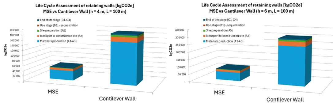
Figure 14: LCA comparison between MSE and Cantilever Wall for two sections (left: 4 m high, 100 m long wall; right: 6 m high, 100 m long wall).
