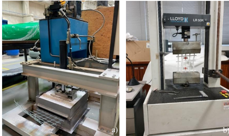
Figure 11: Laboratory tests: a) mechanical damage simulation test; (b) tensile strength test.
