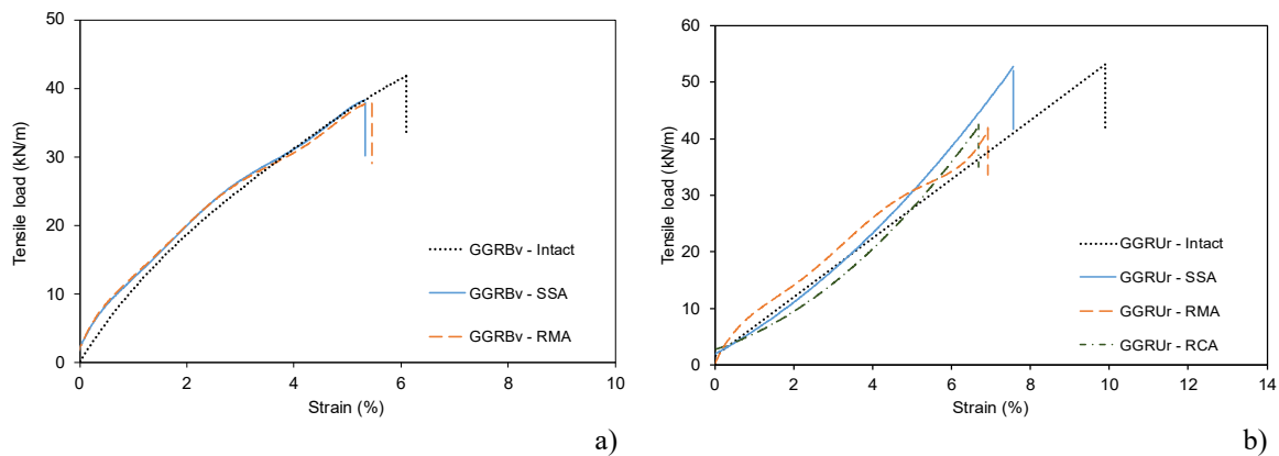
Figure 12: Short-term tensile behaviour of intact and damaged geosynthetic specimens: a) GGRBv (virgin polymer geogrid); b) GGRUr (recycled polymer geogrid).
