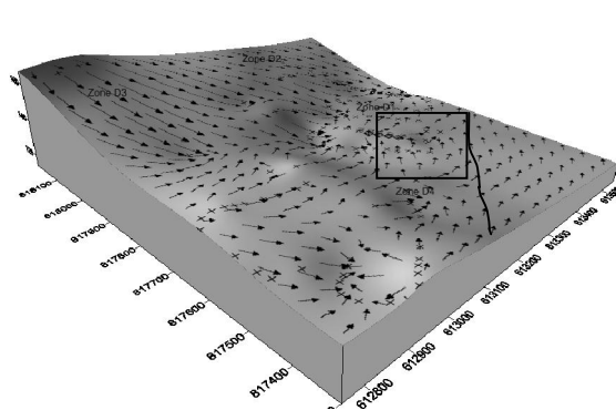
Figure 3b. Destination of infiltrated water over surface of clay layer.
