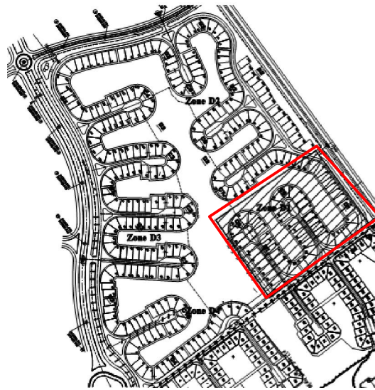
Figure 3c. Marked destination area of surface and infiltrated water on top of clay layer under the layout of the villas in the site.
