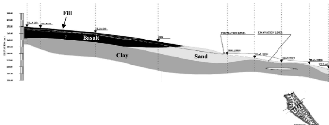
Figure 2a. Geological cross section.
