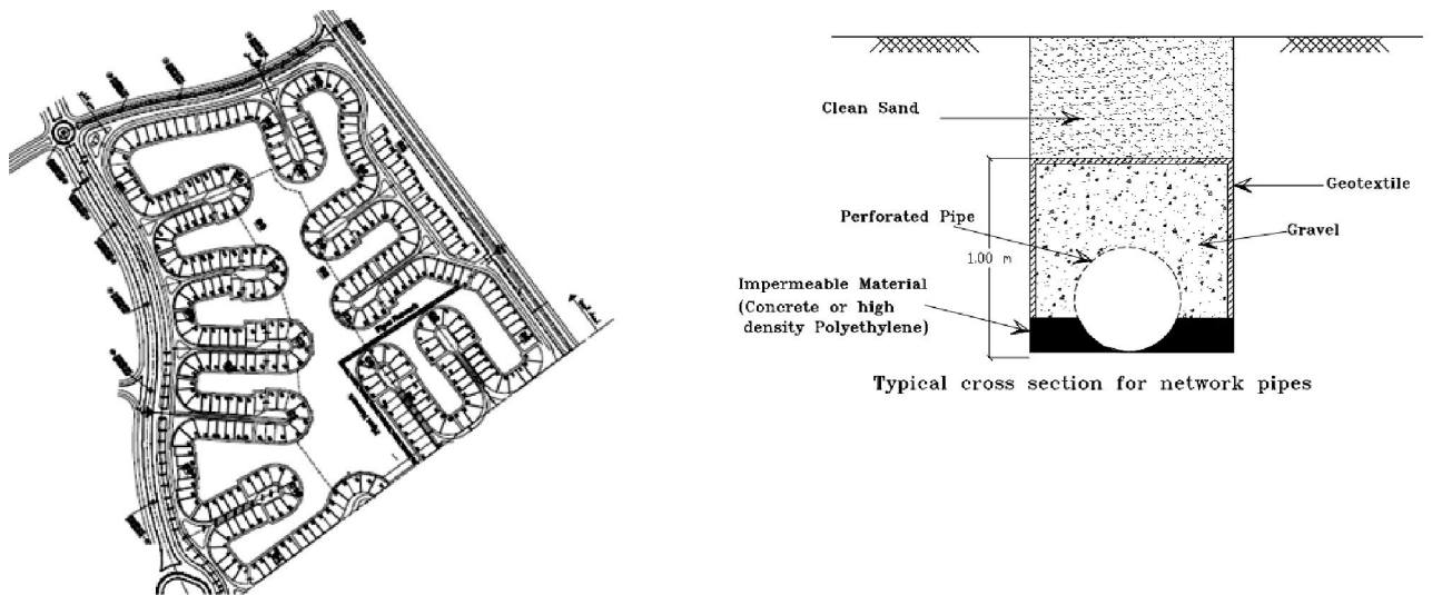
Figure 6. Deep network of perforated pipes
