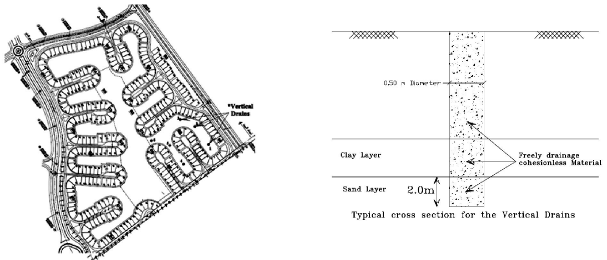
Figure 5. Vertical gravel drains
