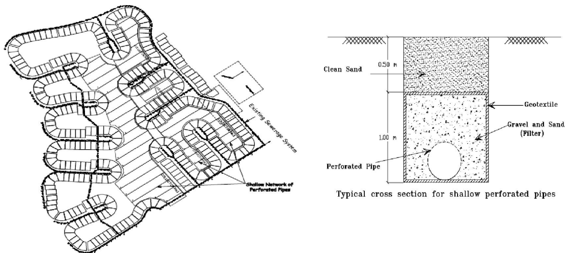
Figure 4. Shallow network of perforated pipes
