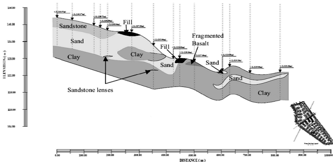
Figure 2b. Geological cross section.
